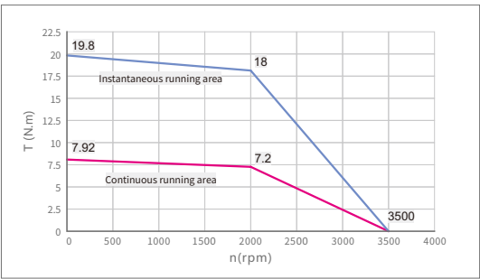
SMC130D-0150-20G□K-4HSP SMS130D-0150-20K□K-4HHP AC380V/ 1.5kW
