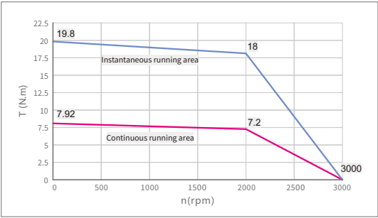
SMC130D-0150-20G□K-4LSP SMS130D-0150-20K□K-4LKP AC220V/ 1.5kW
