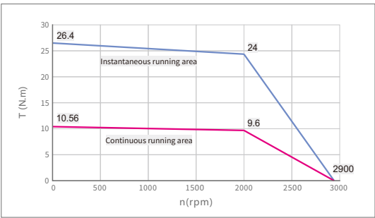
SMC130D-0200-20G□K-4LSP SMS130D-0200-20K□K-4LKP AC220V/ 2kW
