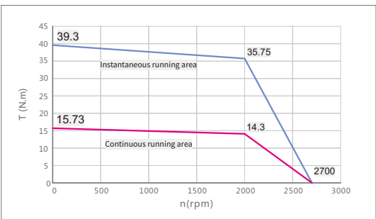
SMC130D-0300-20G□K-4HSP SMS130D-0300-20K□K-4HHP AC380V/ 3kW
