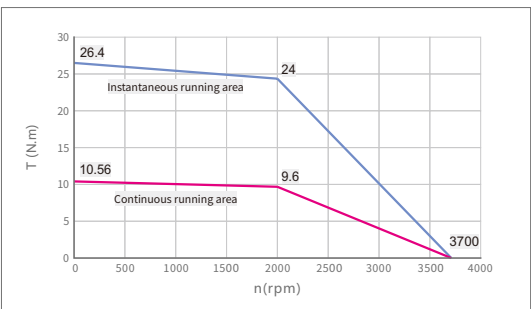
SMC130D-0200-20G□K-4HSP SMS130D-0200-20K□K-4HHP AC380V/ 2kW
