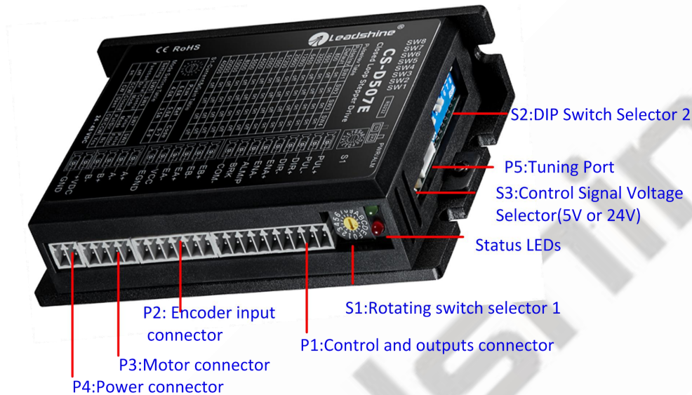
Figure 2: CS-D507E connectors
