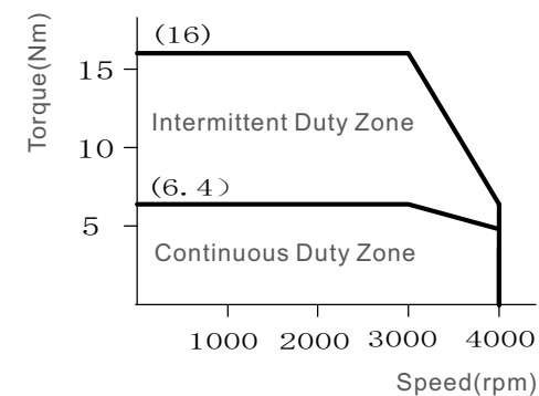
The curve of torque-speed
