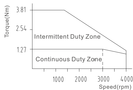
The curve of torque-speed
