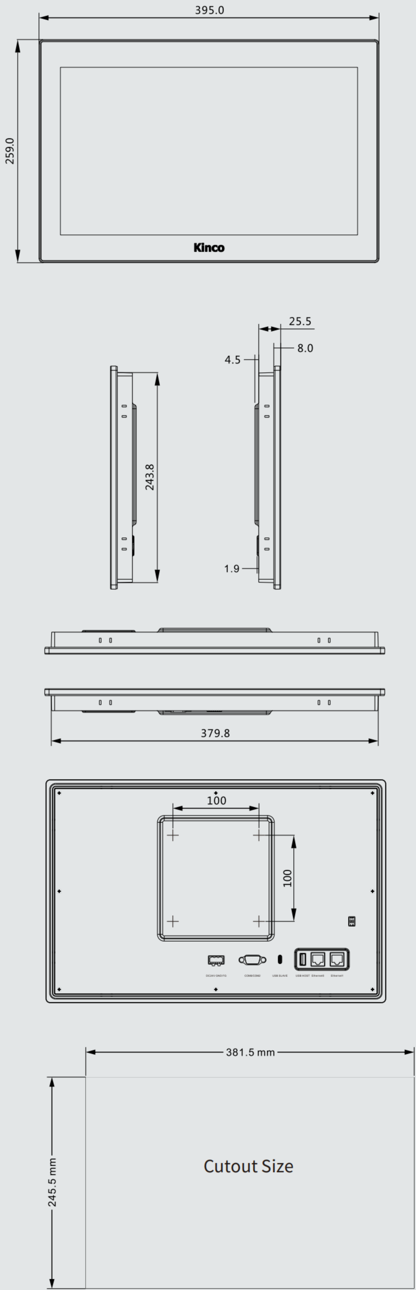
Dimensional diagram (Unit: mm)
