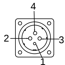
Wiring details of Power cable connector
