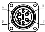
Encoder connector
