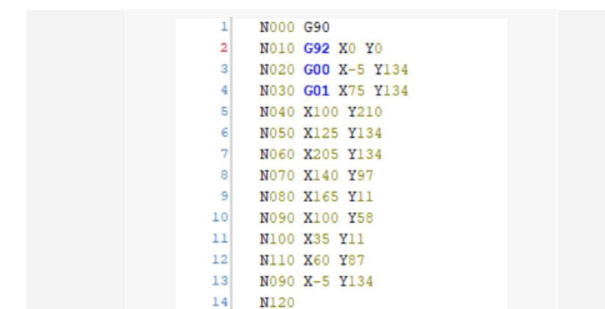
G code
