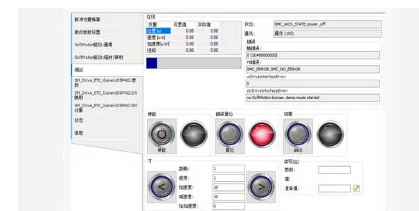
Online simulation
