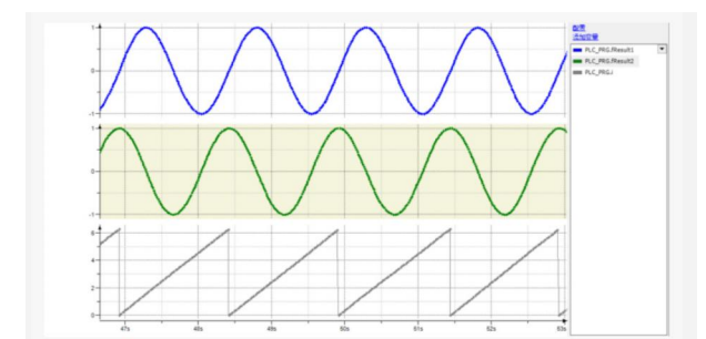
Trace monitor
