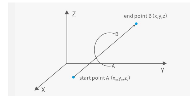
Space Interpolation
